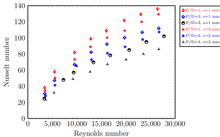
Figure 5. Variation of Nusselt number versus Reynolds number for all configurations.
