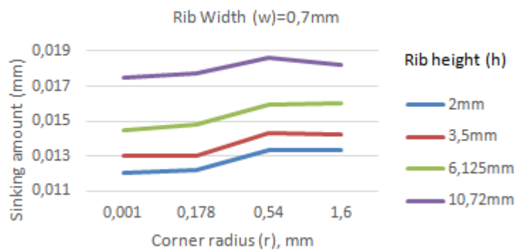
Figure 6. Sinking amounts (Rib width w=0.7mm)
