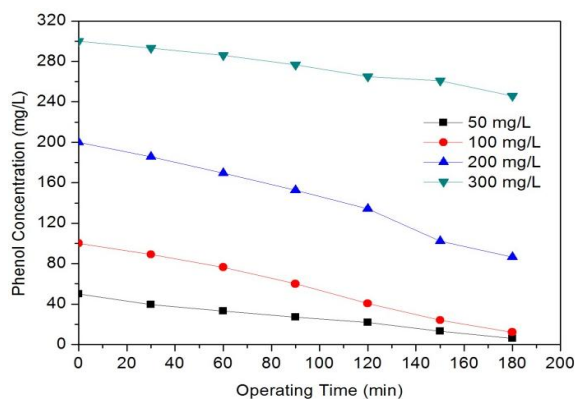
Figure 3.5 The effect of phenol concentration on removal efficiencies (pH=5.0, 2 gr/L \text{Na}_2\text{SO}_4 , 10 mA/cm 2 ).
