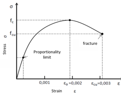
Figure 6 . Typical stress-strain diagram of the Concrete material
