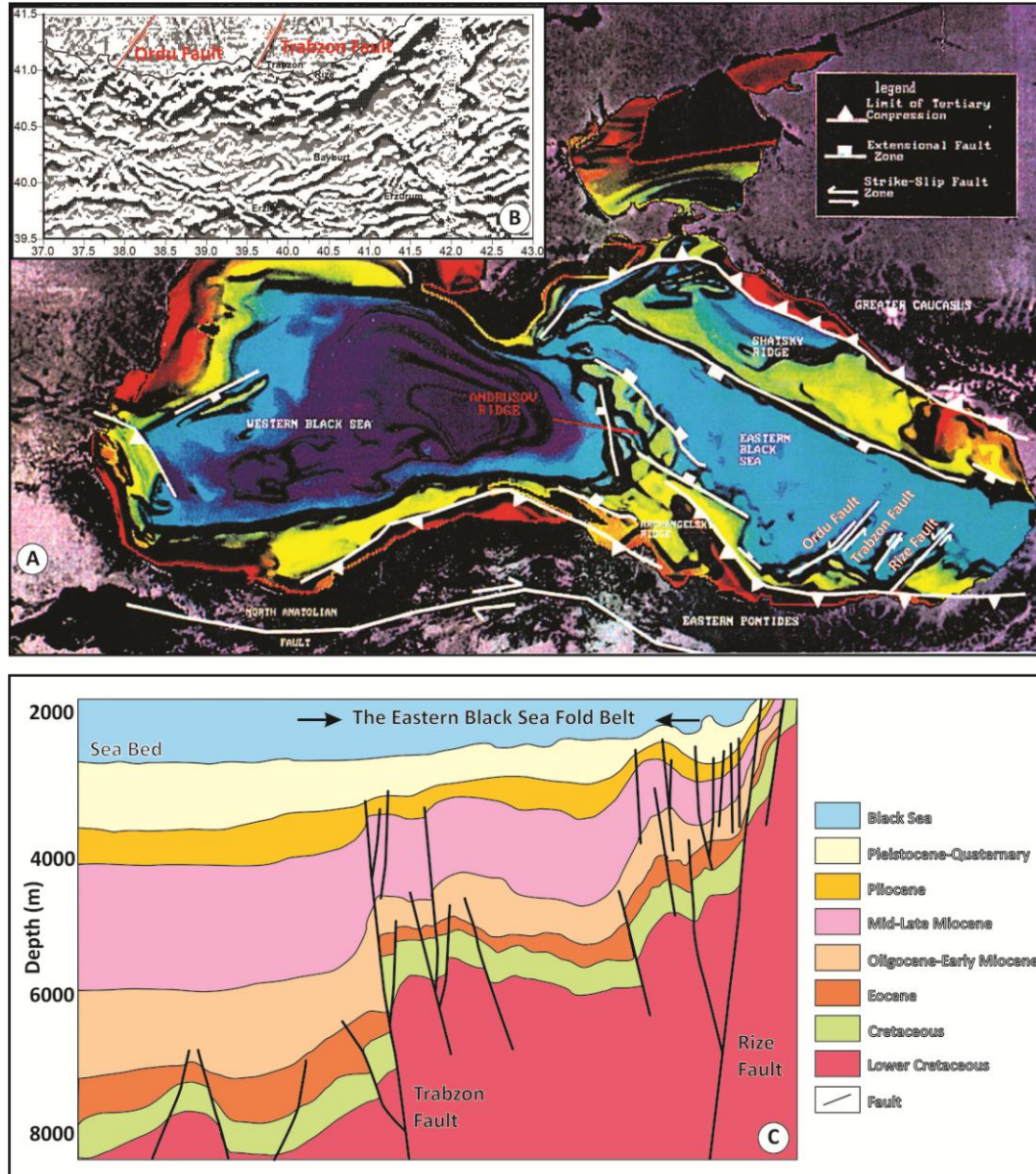
Figure 3. A) Tectonic map of the Black Sea and its vicinity (after [10]) B) Bouguer gravity anomalies map of the eastern Pontides (After [2]). C) Seismic section of the eastern Black Sea (after [10]).
