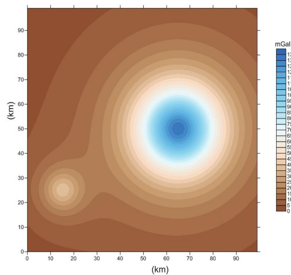
Figure 2. The gravity anomalies of models in Figure 1.
