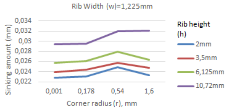
Figure 7. Sinking amounts (Rib width w=1.225mm)
