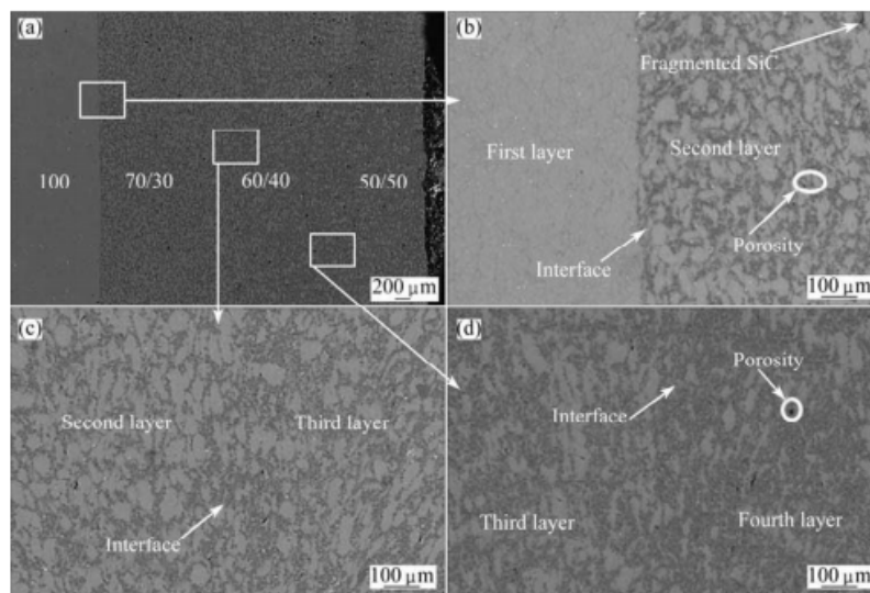
Figure 5. The microstructures of Al2024/SiC functionally graded composites [13]
