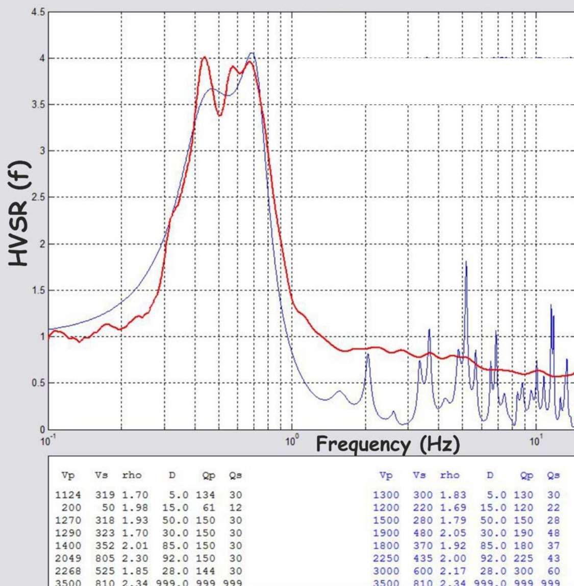
Figure 3. Observational and Theoretical HVSR Comparison ve Ground Model Optimized
