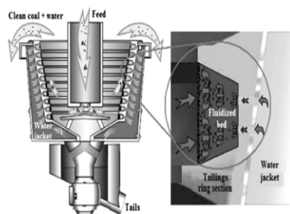
Figure1. Schematic view of the Knelson concentrator [3].
