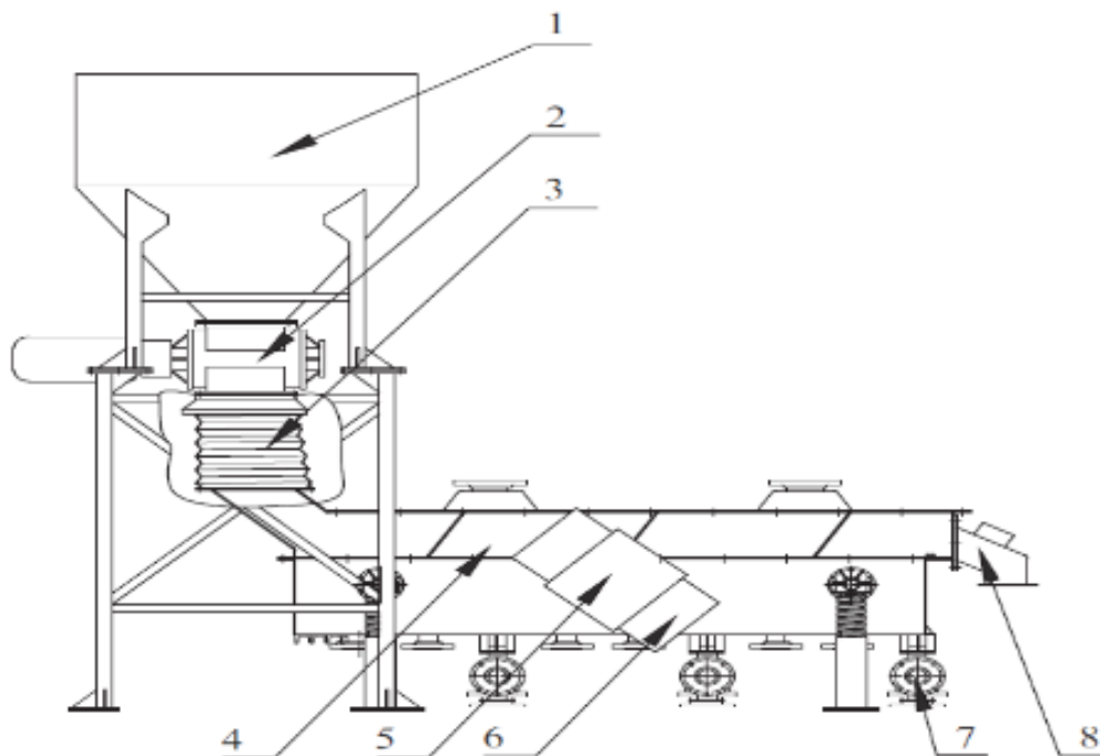
Figure 9. Mechanical structure of the continuous vibrated gas-fluidized bed separator. 1 Feed silo; 2 impeller feeder; 3 flexible coupling materials; 4 separating bed; 5 vibration motor; 6 air chamber; 7 impeller discharging device; 8 overflow discharge opening of clean coal [4].
