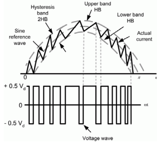
Figure 1. Hysteresis current controller basic scheme
