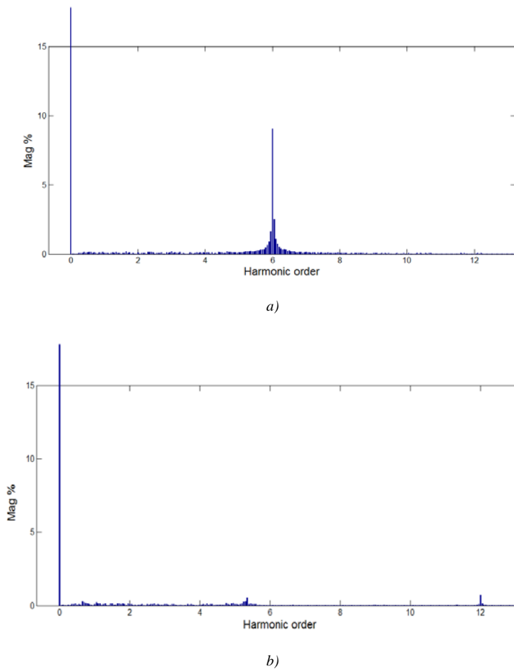
Figure 5. Harmonic spectrum of torque
