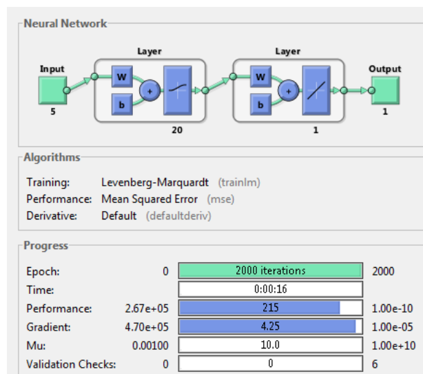
Figure 2. Training network
