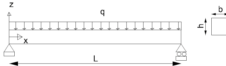
Figure 1. A Simply supported FGM beam subjected to distributed load
