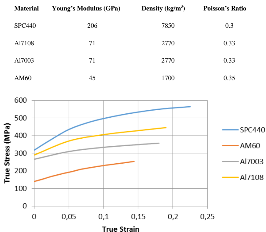
Figure 4. True stress – strain curve of used steel and low density materials
