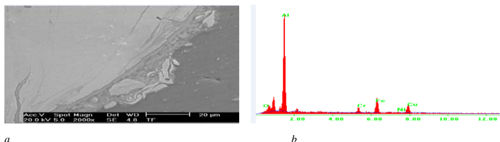
Figure 6. a- Friction stir spot welding interface stir zone of coper coated AA1050 aluminum alloy with AISI 304 welded by FSSW.b- EDS analysis results of friction stir spot welding interface stir zone of coper coated AA1050 aluminum alloy with AISI 304 welded by FSSW.
