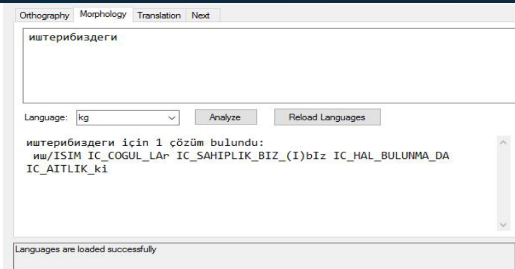
Figure 16. Morphological parsing in NUVE
