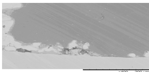
Figure 6. a- Friction stir spot welding interface stir zone of coper coated AA1050 aluminum alloy with AISI 304 welded by FSSW.b- EDS analysis results of friction stir spot welding interface stir zone of coper coated AA1050 aluminum alloy with AISI 304 welded by FSSW.
