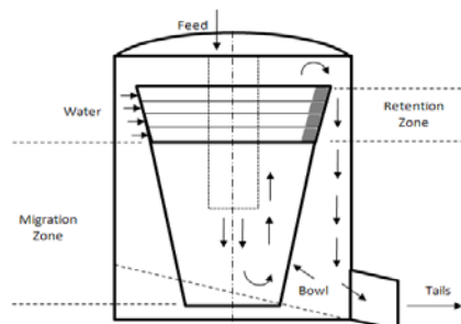
Figure 2. Schematic view of a Falcon Centrifugal Concentrator [13].
