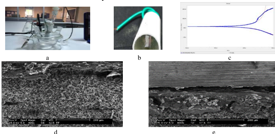
Figure 10. a- Corrosion measurement device b- Corrosion measurement sample c- Potentiodynamic polarization Tafel curves of welded interface regions along with the BM d,e- The general welded zones after corrosion test along with the BM and interface SEM micrograph
